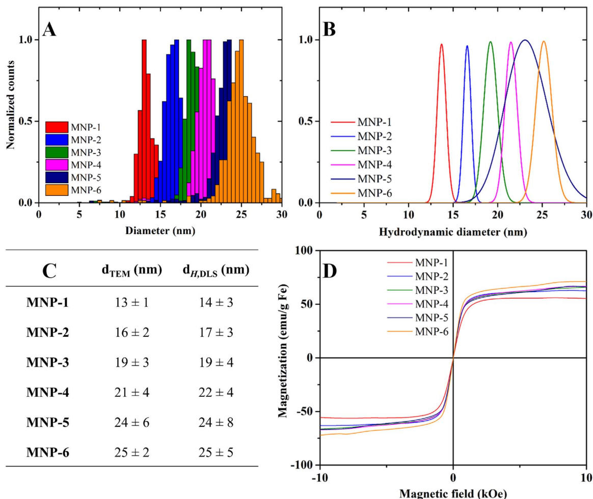
Fig. 3. Size and magnetic characterization of MNPs. Size histograms were determined by TEM micrographs (A). Nanoparticle stability and hydrodynamic diameter ( d_H ) were determined via DLS (B). A summary table shows the core diameter measured by TEM and d_H measured by DLS (C). Sizes represent mean \pm SD. Vibrating sample magnetometry highlighted the superparamagnetic nature of the MNPs (D).
